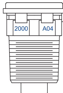
Typical 1" Snap-on gauge head Model B8900-02000
